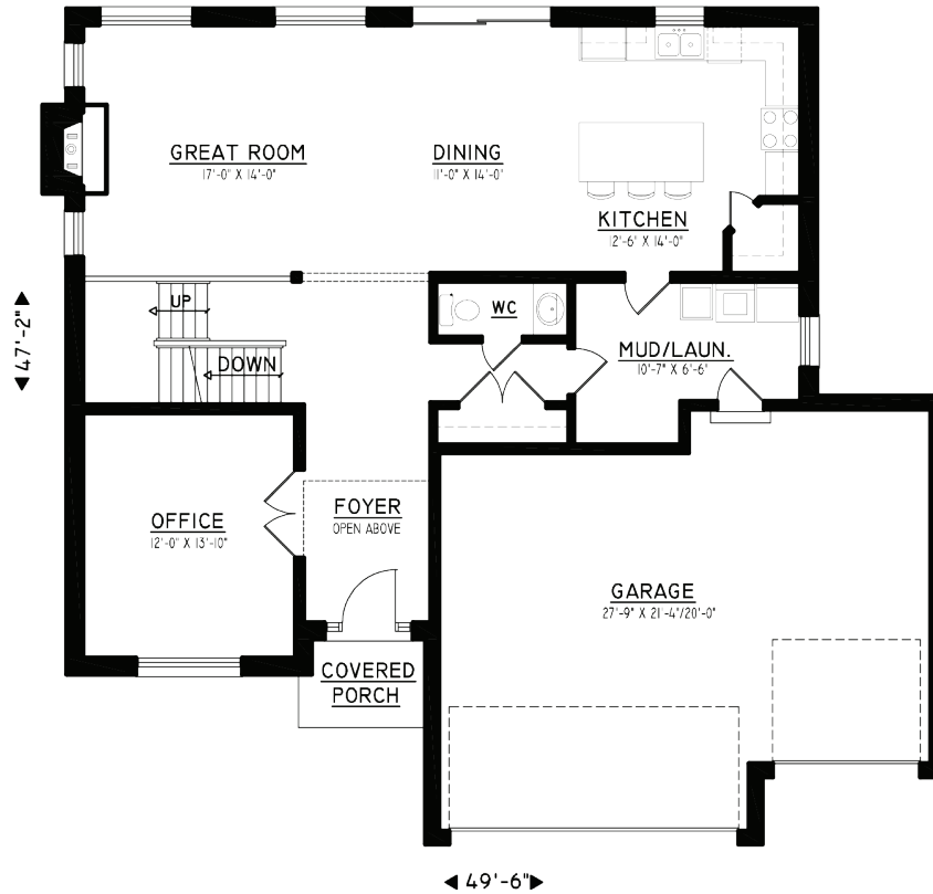
MAIN FLOOR PLAN TOTAL APPROX. - 1296 SQ. FT.
