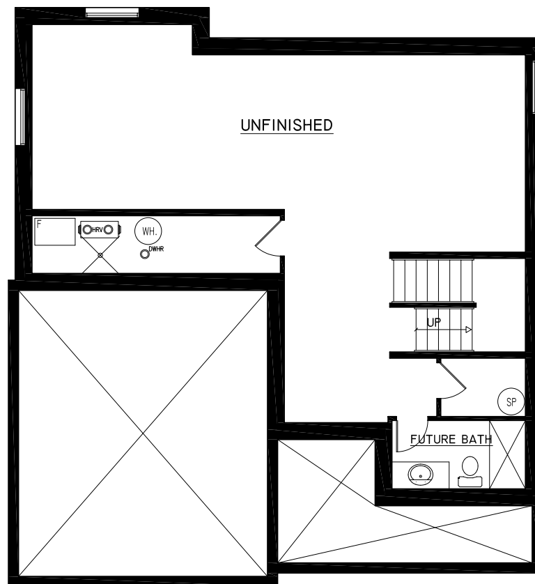
BASEMENT PLAN
