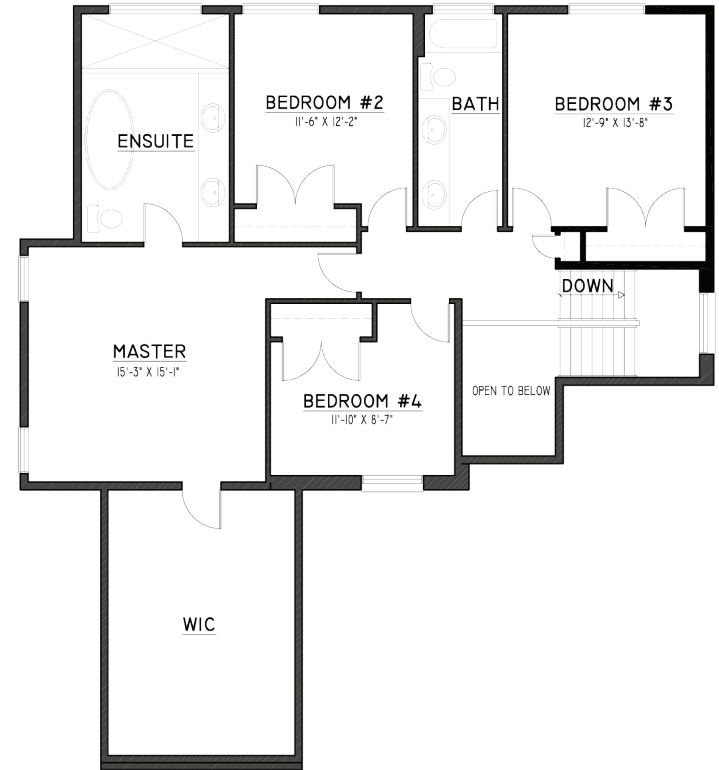
SECOND FLOOR PLAN (4 BEDROOM OPTION) TOTAL APPROX. - 1378 SQ. FT.
