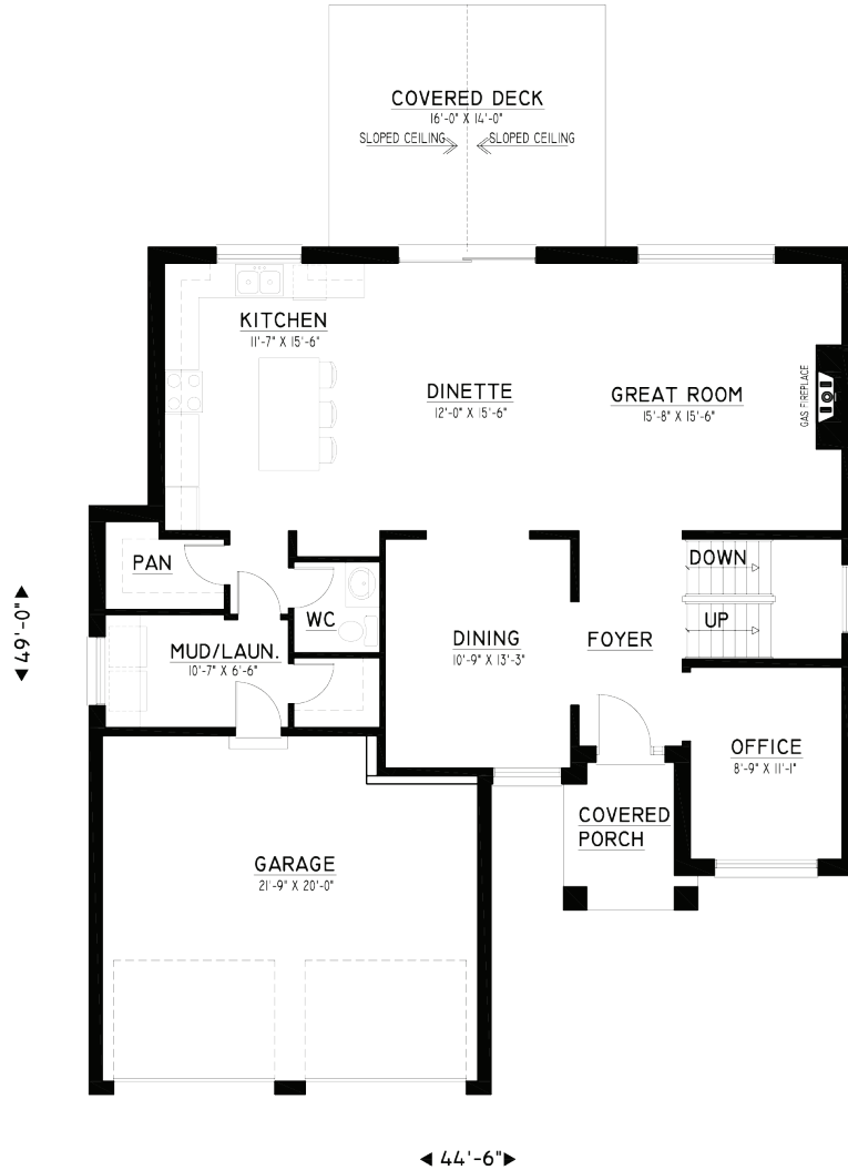
MAIN FLOOR PLAN TOTAL APPROX. - 1339 SQ. FT.
